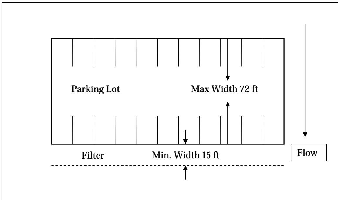
Figure 5-14: Example configuration of filter strip adjacent to parking lot in plan view.
