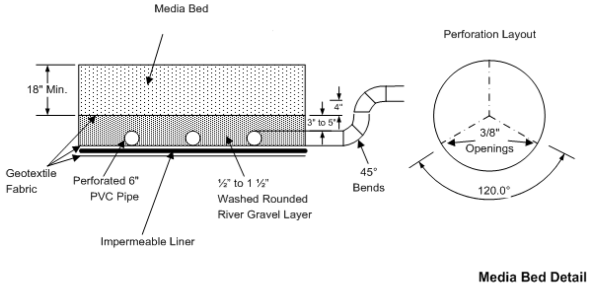
Figure 5-9: Illustration of optional outlet design
