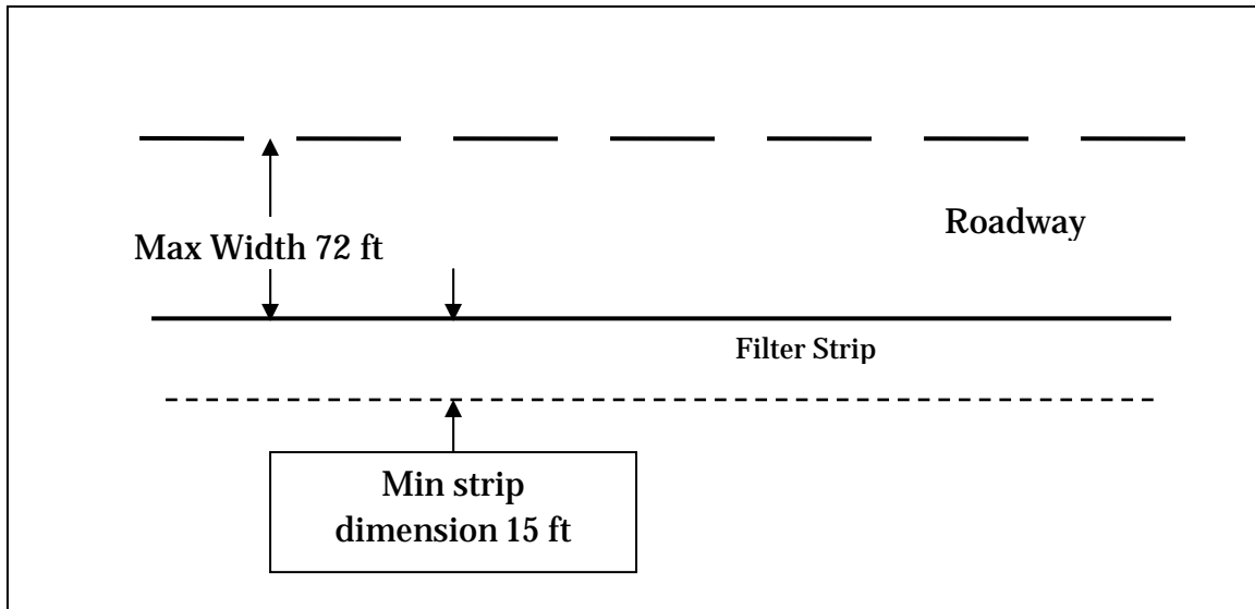
Figure 5-13: Example of filter strip along roadway in plan view.
