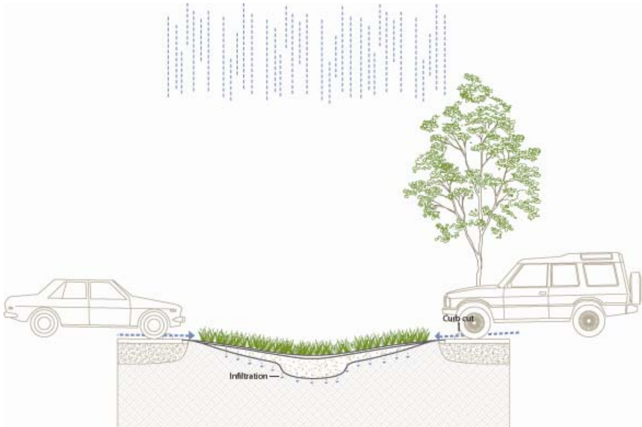
Figure 4-6: Swale in parking lot area showing the use of short grasses, low slopes, curb cuts from parking area and some infiltration.
