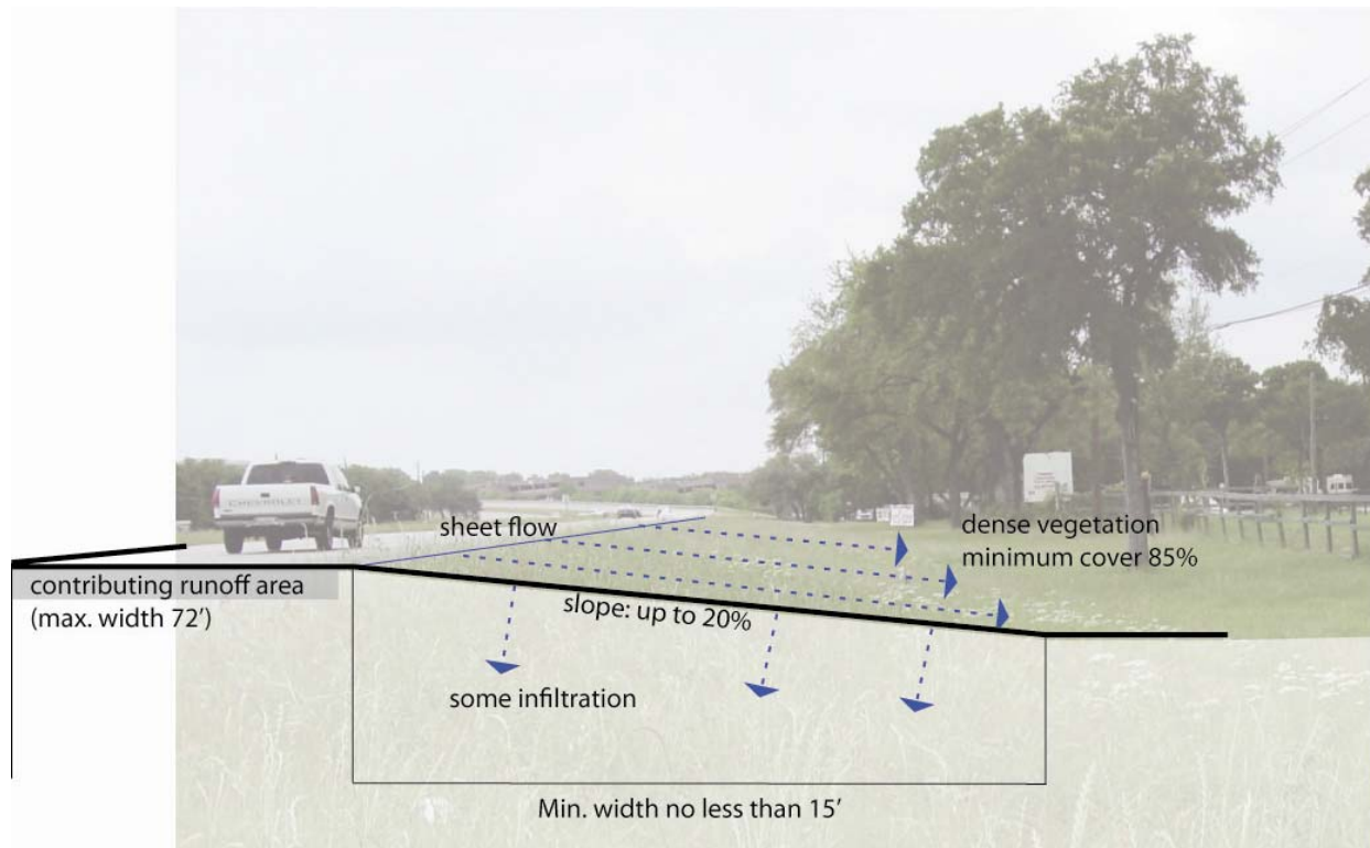
Figure 5-12: Engineered VFS in context.
