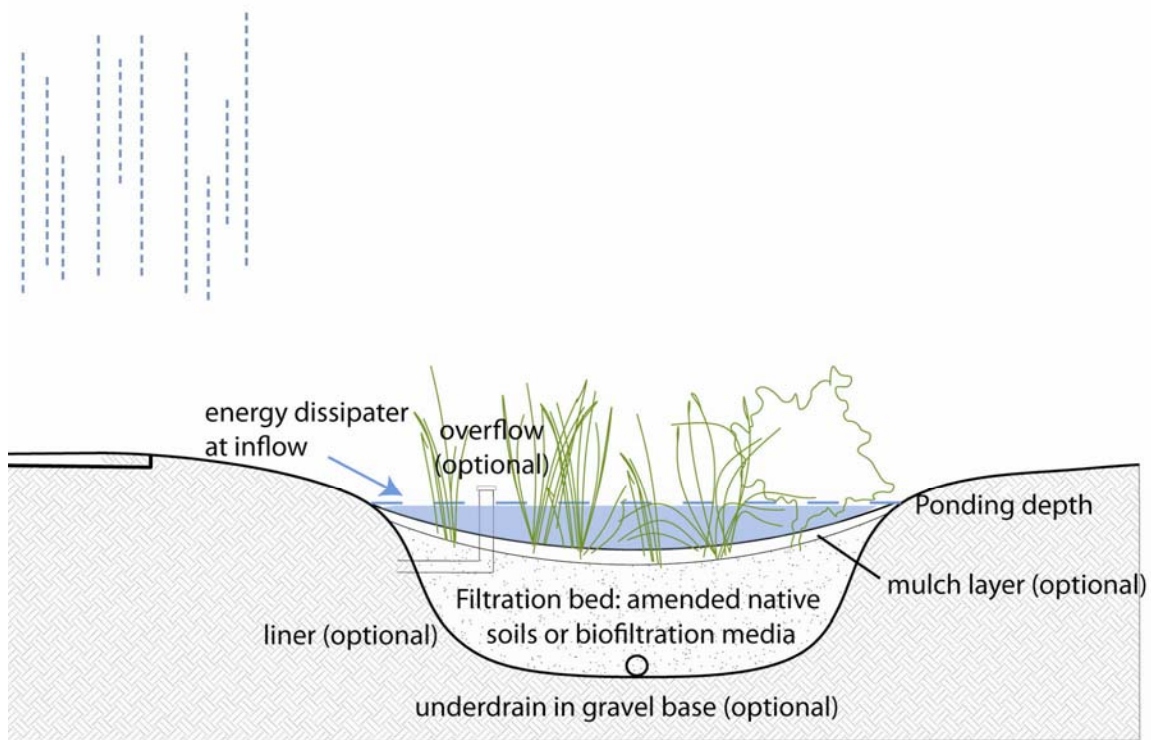
Figure 4-1: A diagram of the basic rain garden / bioretention system components, including optional components.
