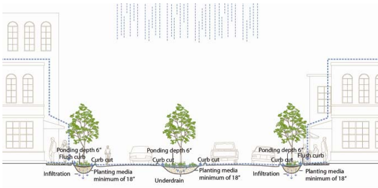
Figure 5-4: Bioretention along streets with a combination of infiltration and underdrain.
