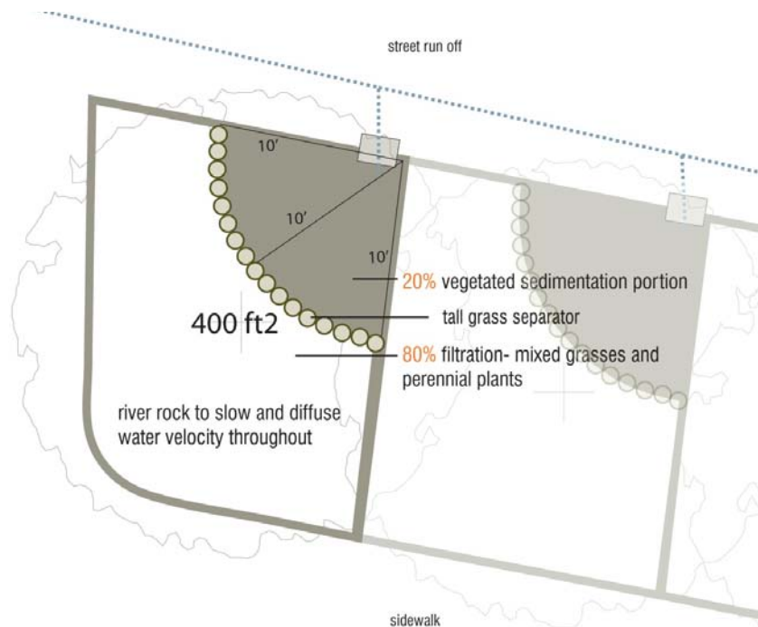
Figure 5-2: An example of a rain garden design following City of Austin specifications as described in Section 1.6.7 of the Environmental Criteria Manual (2009).
