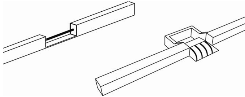
Figure 5-7: Curb cuts with optional sediment / trash screens
