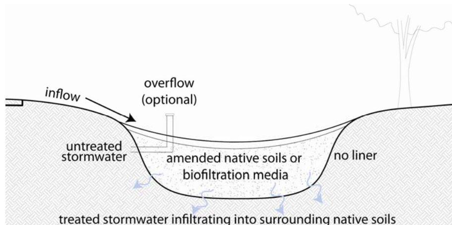
Figure 5-3: Rain garden schematic with no underdrain.
