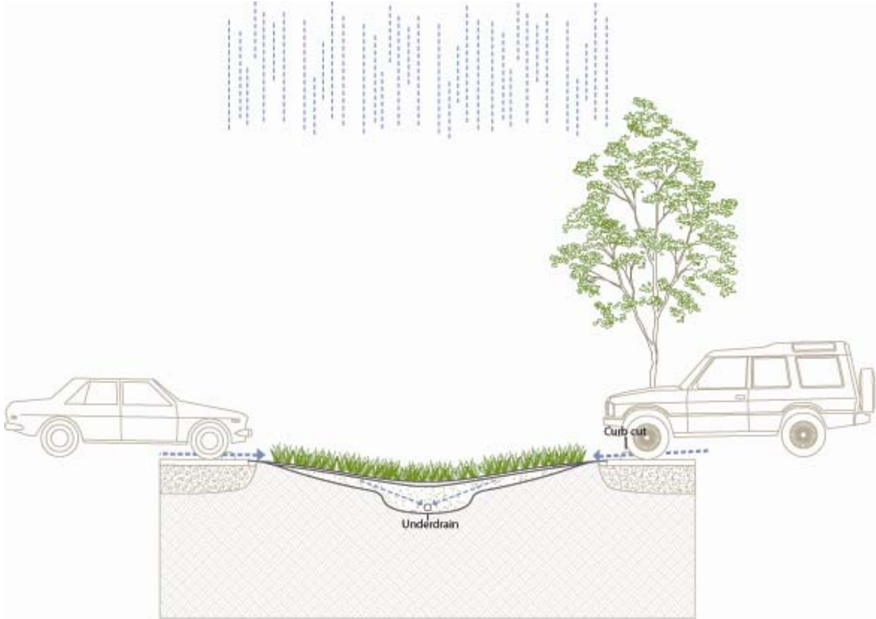
Figure 5-11: Enhanced swale diagram with underdrain system in parking lot.
