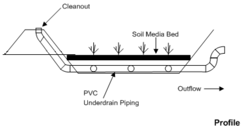
Figure 5-8: Detail of cleanout location
