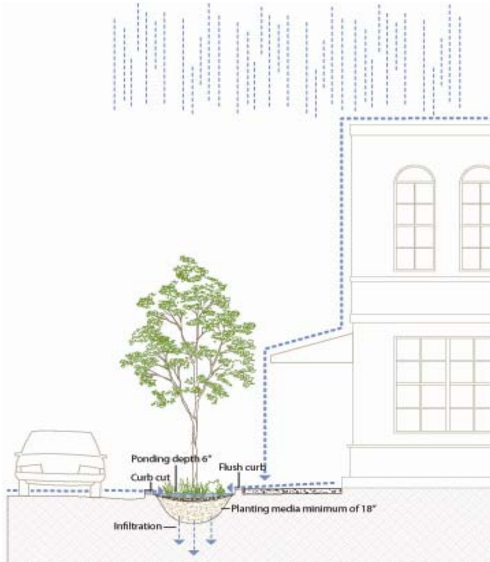
Figure 4-4: Schematic of a bioretention/rain garden BMP with no underdrain; treated stormwater infiltrates into surrounding soils.
