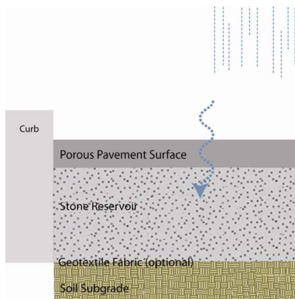
Figure 5-15: Basic components of a porous pavement system.
