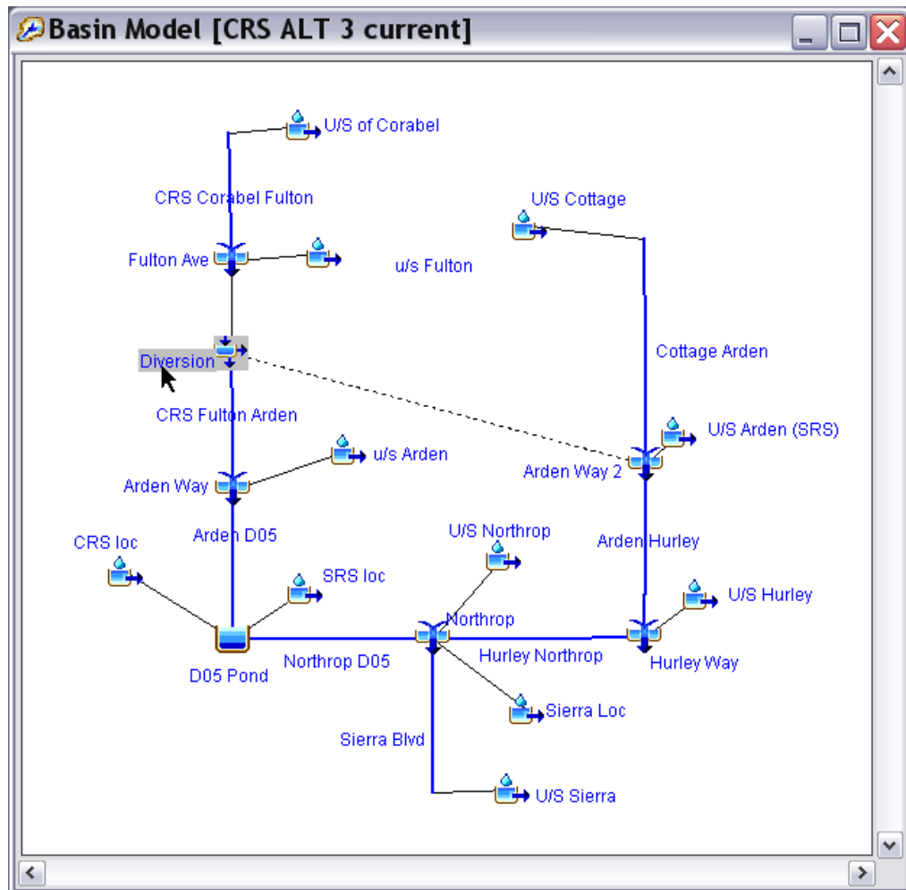
Figure 28. Basin model for alternative 3.
