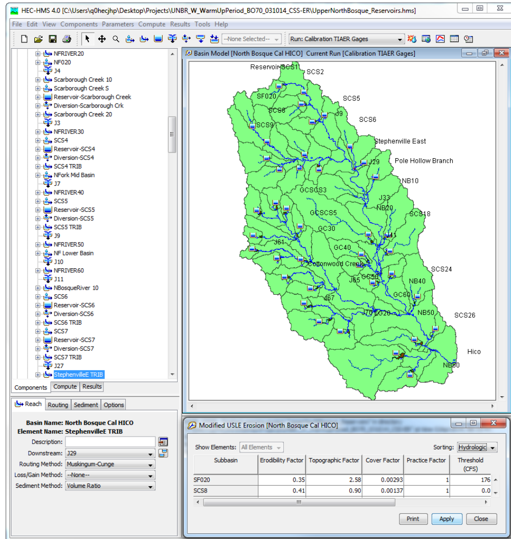
Figure 55. Sediment model set up in HEC-HMS.
