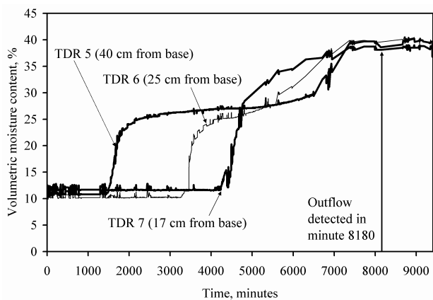
Figure 5: Volumetric moisture content with depth in Profile 2
