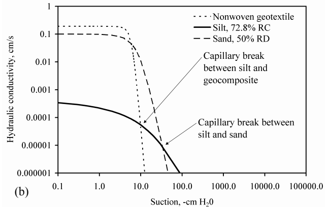
Figure 2: Soil and geocomposite hydraulic characteristics: (a) Water characteristic curve; (b) Hydraulic conductivity functions (K-functions)
