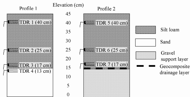
Figure 3: Schematic of soil profiles
