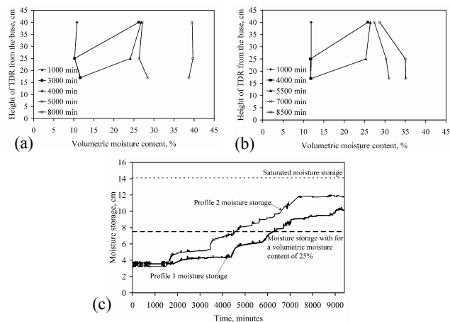
Figure 6: (a) Moisture profiles in Profile 1 (silt-sand); (b) Moisture profiles in Profile 2 (silt-geocomposite); (c) Water storage in Profiles 1 and 2 at flow equilibrium and at saturation
