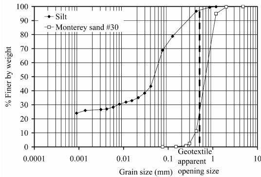
Figure 1: Comparison between the silt and Monterey sand #30 grain size distributions and the geotextile apparent opening size
