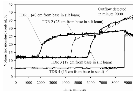
Figure 4: Volumetric moisture content with depth in Profile 1
