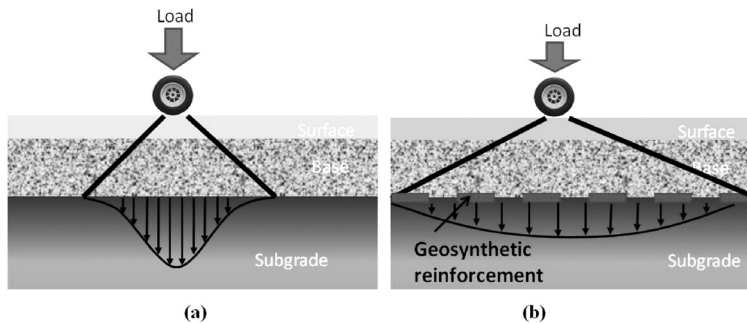
Fig. 2 Relative load magnitudes at subgrade layer level for (a) unreinforced flexible pavement and (b) geosynthetic-reinforced flexible pavement
