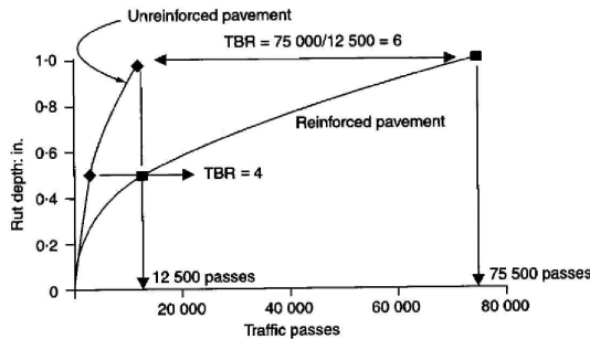
Fig. 4 Typical TBR values for an unreinforced and reinforced pavement to reach a given rutting depth (Shukla 2002)
