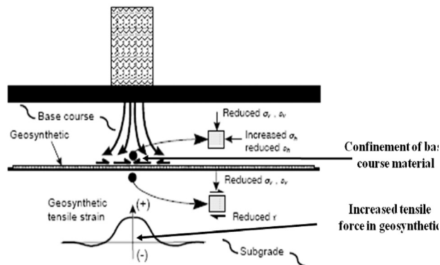
Fig. 7 Mechanisms due to soil-geosynthetic interaction in geosynthetic-reinforced pavement that have been tried to be represented in laboratory tests (Perkins 1999)
