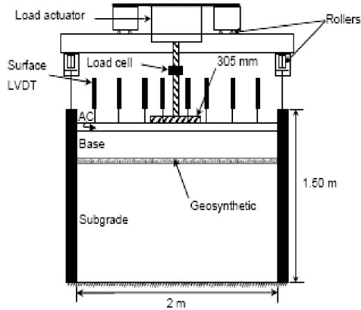
Fig. 9 Cyclic plate load test (Perkins 1999)
