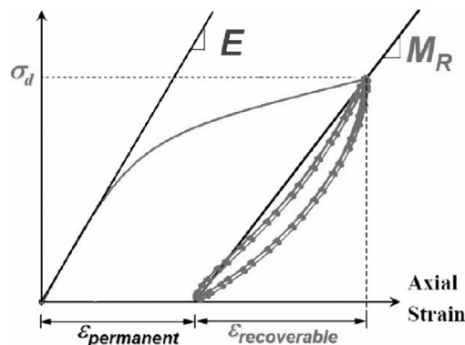
Fig. 5 Comparison of Resilient Modulus, M_R , and Modulus of Elasticity, E
