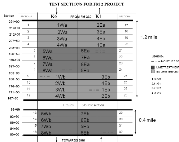
Fig. 6 Schematic layout of test sections at FM 2 site
