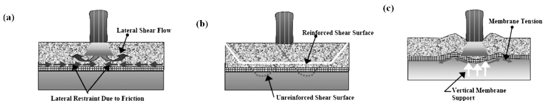
Fig. 3 Reinforcement mechanisms induced by geosynthetics (Holtz et al. 1998): (a) Lateral restraint; (b) Increased bearing capacity; and (c) Membrane support
