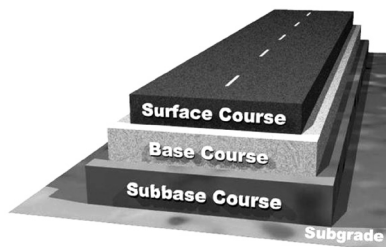
Fig. 1 Cross-section of flexible pavement system (Muench 2006)
