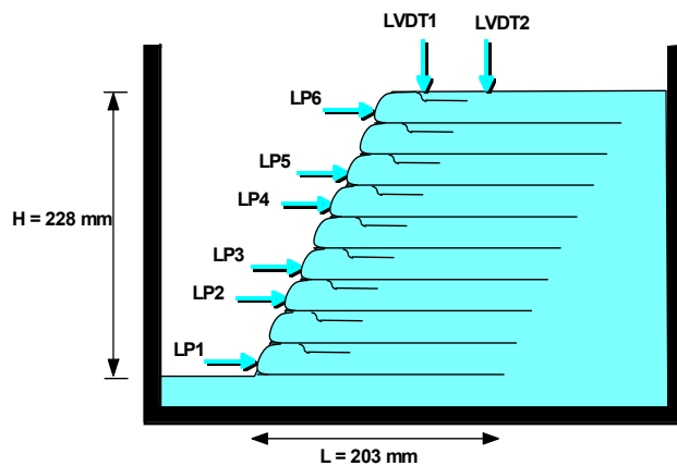
Figure 1. Typical centrifuge model.
