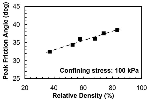
Figure 3. Friction angle for Monterey No. 30 sand obtained from triaxial testing at different relative densities.
