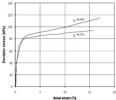
Figure 18 Stress-strain behavior of specimens prepared using \chi_w=0.2, 0.4\% , with l=25 mm fibers (2610 denier), \sigma_3=116 kPa, Soil 2
