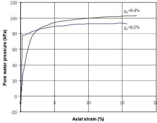
Figure 19 Excess pore water pressure of specimens prepared using \chi_w = 0.2, 0.4\% , with l=25 mm fibers (2610 denier), \sigma_3=116 kPa, Soil 2
