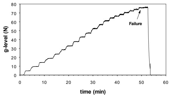
Figure 4. G-level (N) versus time during centrifuge testing.
