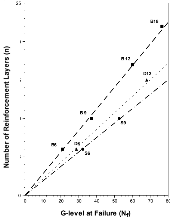
Figure 8. G-level at failure for the centrifuge models. The higher peak soil shear strength in this test series.
