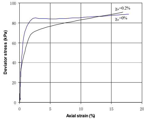
Figure 16 Stress-strain behavior of specimens prepared using \chi_w=0, 0.2 \% , with l=50 mm fibers (2610 denier), \sigma_3=98 kPa, Soil 2
