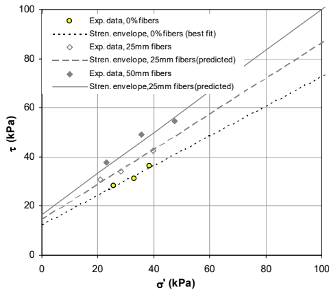
Figure 23 Comparison between predicted and experimental shear strength results for specimens reinforced at \chi_w = 0.4\% , with 25 mm-long and 50 mm-long fibers (2610 denier), Soil 2
