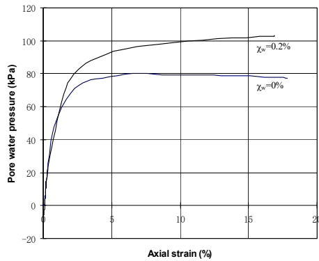
Figure 17 Excess pore water pressure of specimens prepared using \chi_w=0, 0.2 \% , with l=50 mm fibers (2610 denier), \sigma_3=98 kPa, Soil 2
