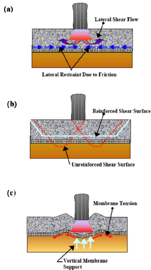
Figure 3: Reinforcement mechanisms induced by geosynthetics (Holtz et al. 1998): (a) Lateral restraint; (b) Increased bearing capacity; and (c) Membrane support
