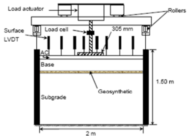
Figure 9: Cyclic plate load test (Perkins 1999)
