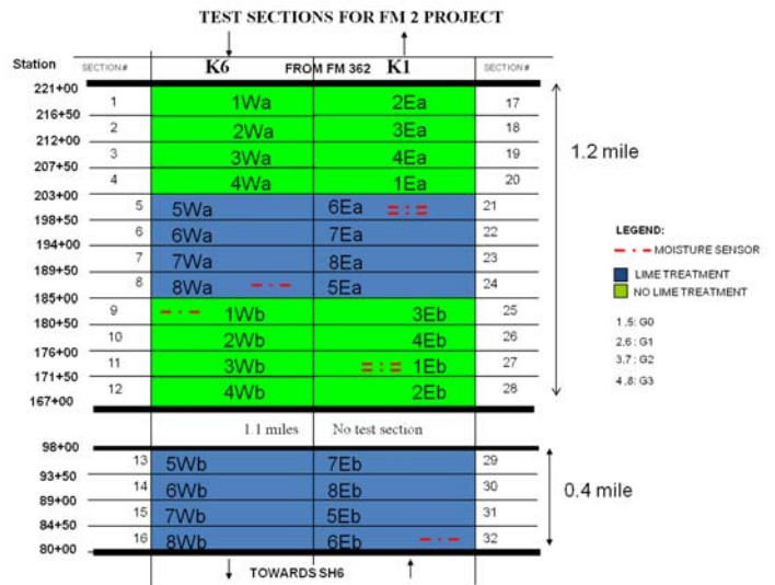
Figure 6: Schematic layout of test sections at FM 2 site
