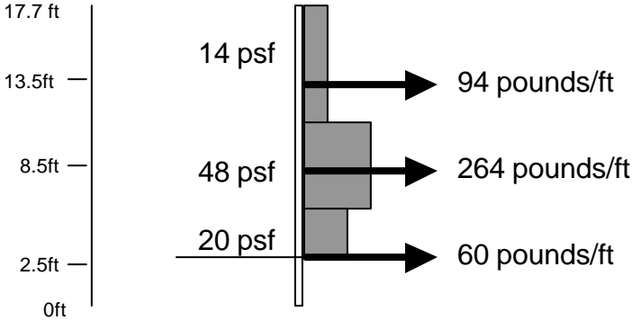
Figure 5.9. Average Anchor Forces and Earth Pressures along Panels of Station 3116.
