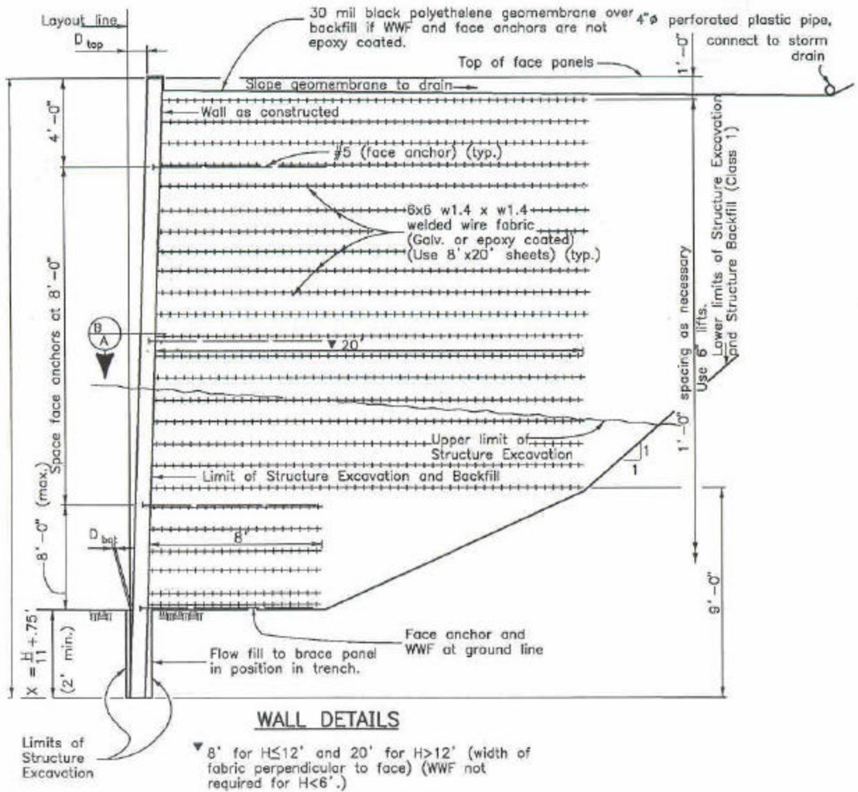
Figure 2.2 Details of the I-25/I-70 MSE/IFF Wall (from Construction Plans)
