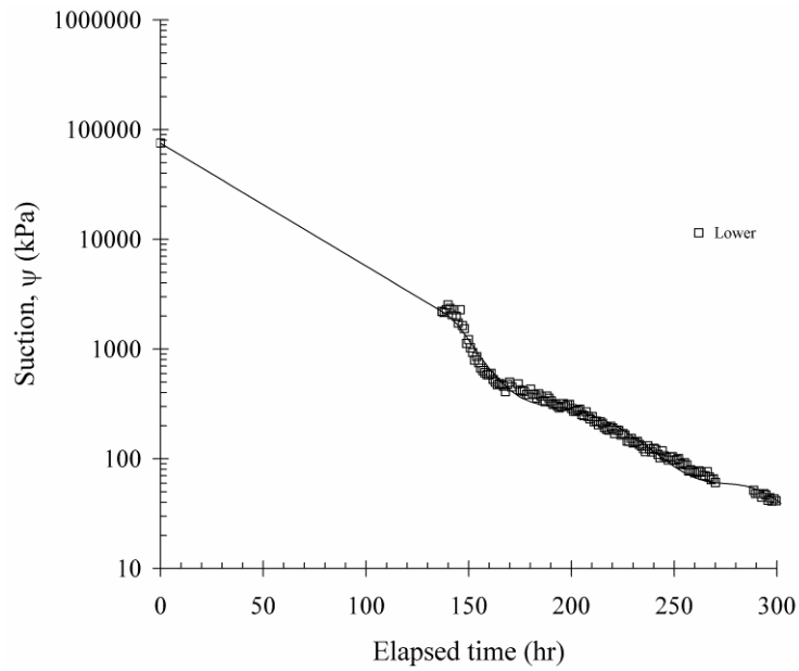
Figure 4.33: Suctions in Soil Column 4 during infiltration phase obtained using HDU measurements
