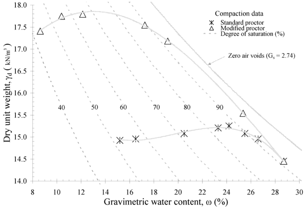
Figure 3.2: Compaction curves for Eagle Ford clay
