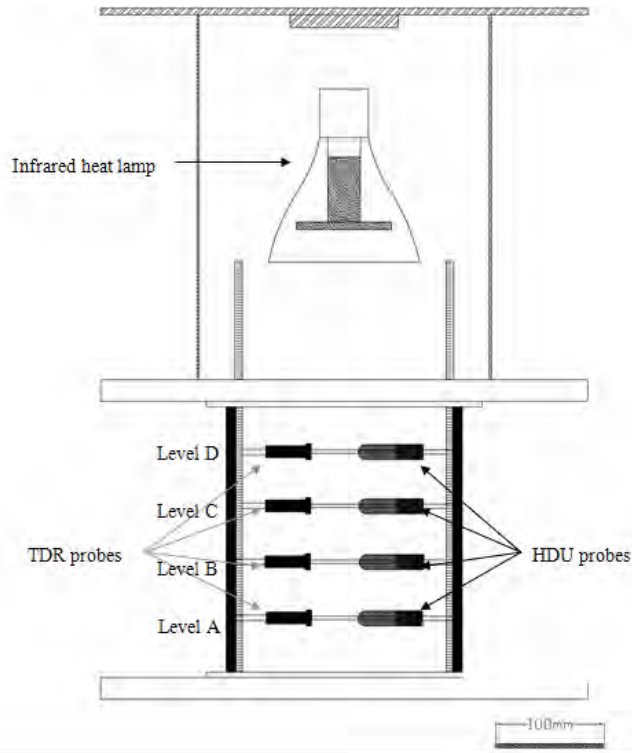
Figure 3.8: Instrumentation setup for Soil Column 3 drying phases
