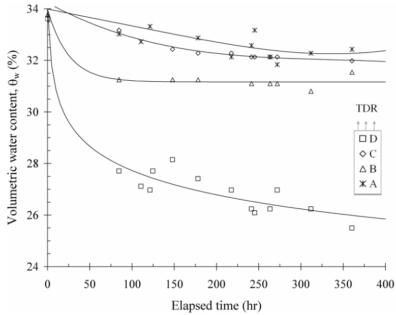
Figure 4.15: Volumetric water contents in Soil Column 3 during first evaporation phase obtained using TDR measurements
