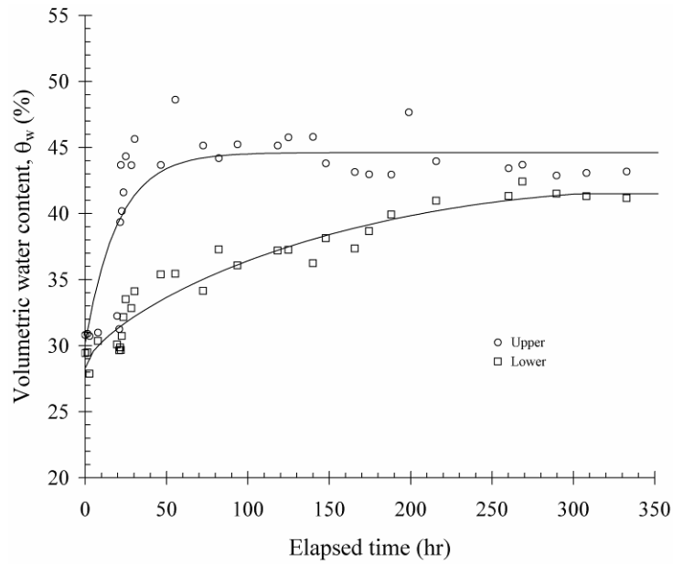
Figure 4.32: Volumetric water content in Soil Column 4 during infiltration phase obtained using TDR measurements
