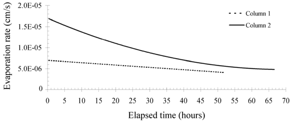
Figure 5.5: Evaporation rates from Soil Column 1 and Soil Column 2
