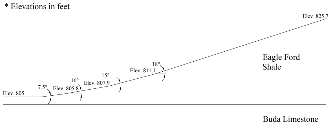
Figure 8.1: Slope geometry used during stability analyses.
