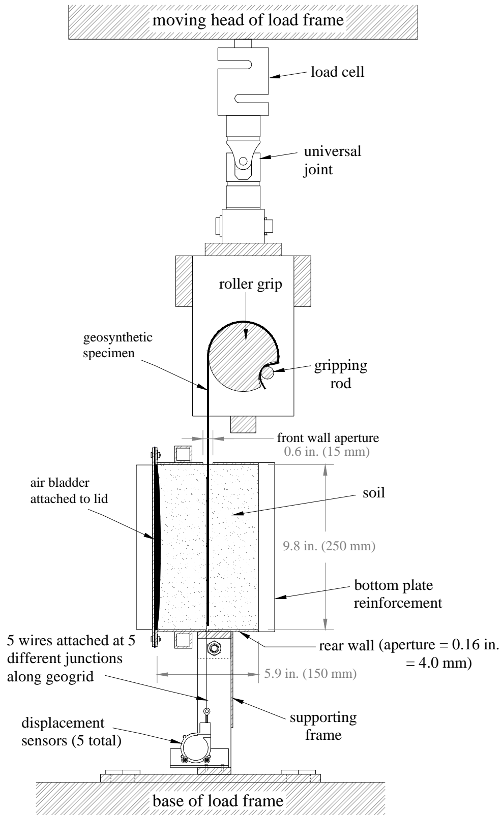
Figure 2.1 Cross section of the small pullout test setup.
