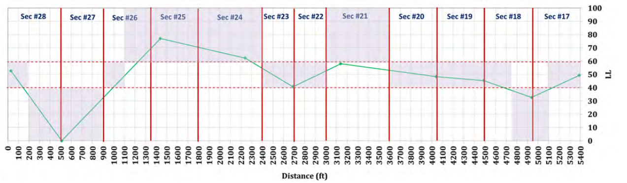
Figure 3.39 LL value for the surface layers of soil.
