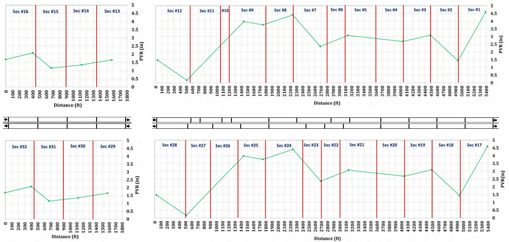
Figure 3.40 PVR value calculated from the surface to the bottom of the borings.
