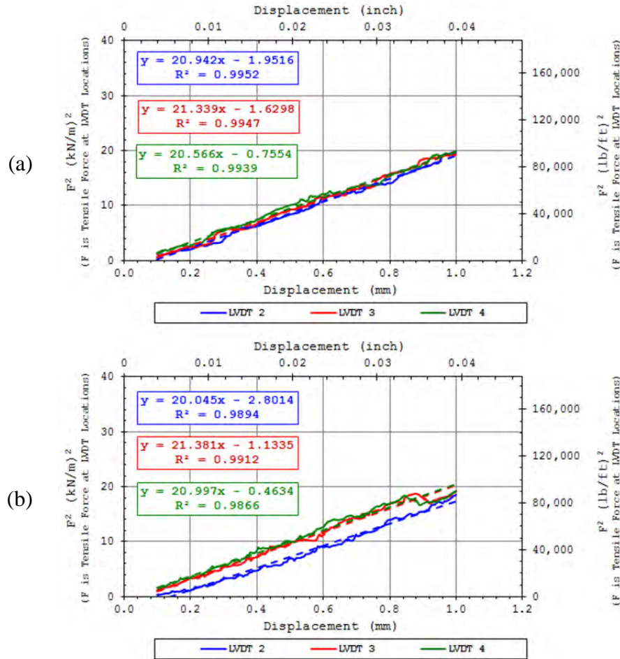
Figure 2.9 K_{SGI} plots for repeat tests of GG PP CD in Monterey Sand, confining pressure of 3.0 psi controlled by an analog pressure gauge and use of torque equal to 12.5 lbf/ft.
