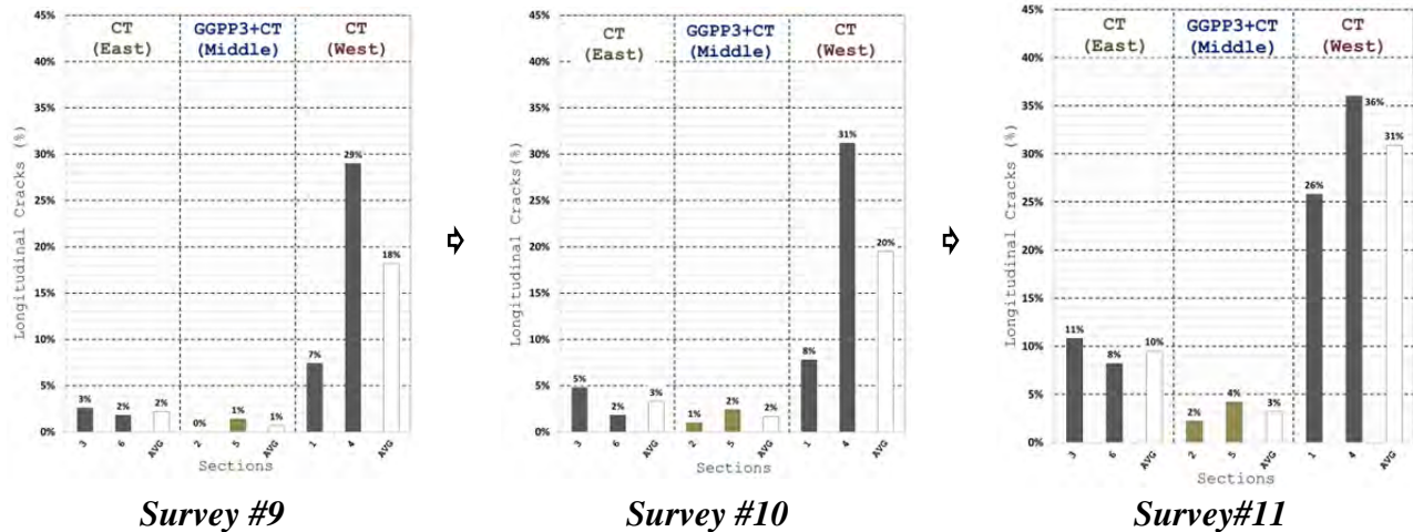
Figure 3.54 Comparison of the performance of the FM1644 test sections over time.
