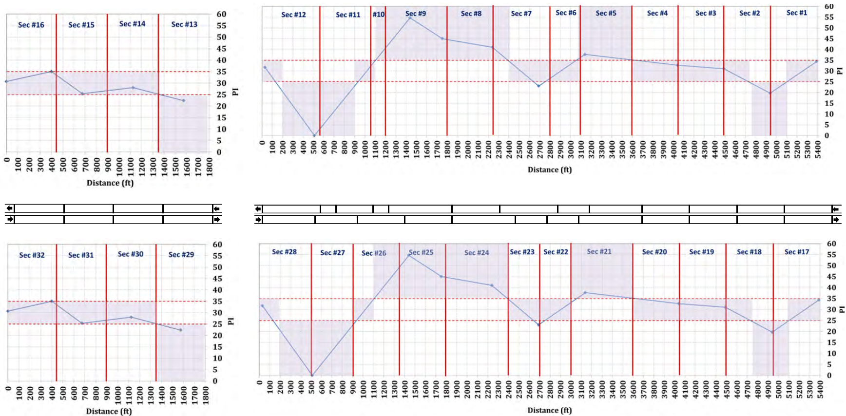
Figure 3.38 PI value for the surface layers of soil.
