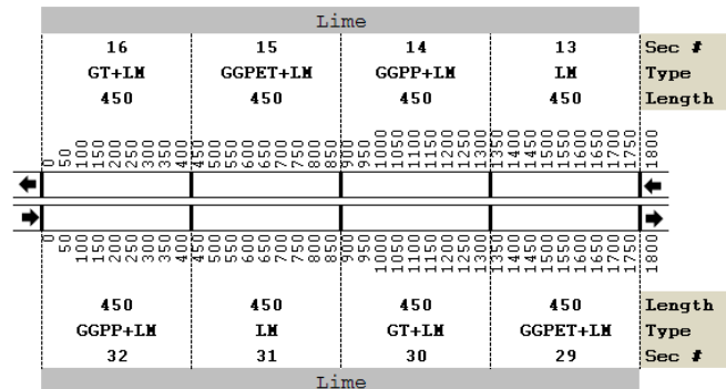
Figure 3.18 The final layout of FM2 test sections.
