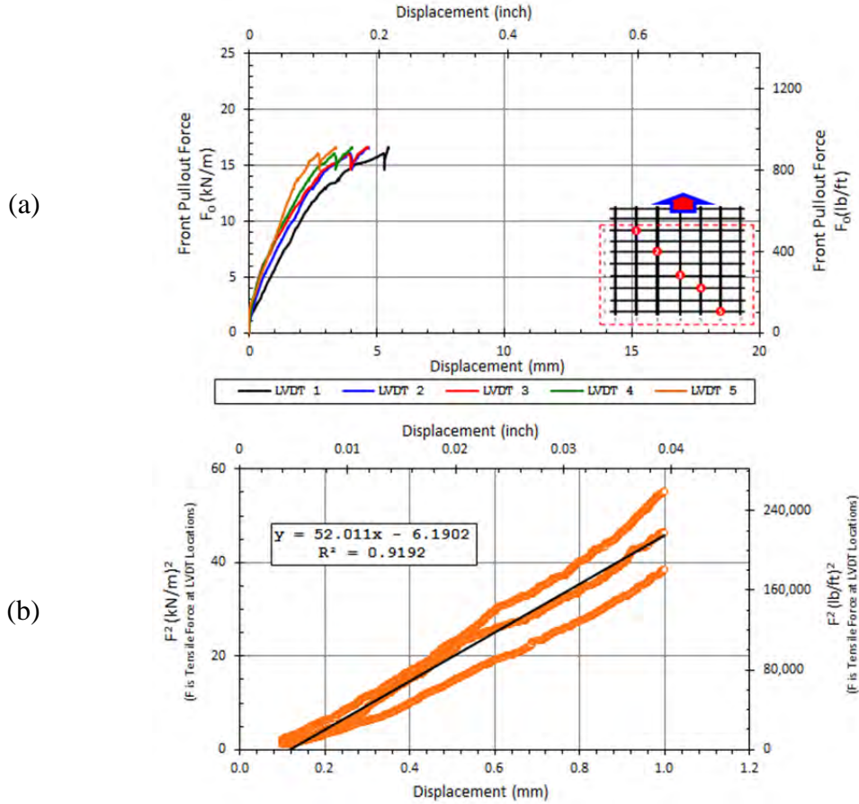
Figure 2.12 Pullout test with Aggregate and GG PET CD with occurrence of particle jamming at the front wall aperture of the box: (a) Pullout curve; (b) K_{SGI} plot: K_{SGI} = 52.0 (\text{kN/m})^2/\text{mm} .
