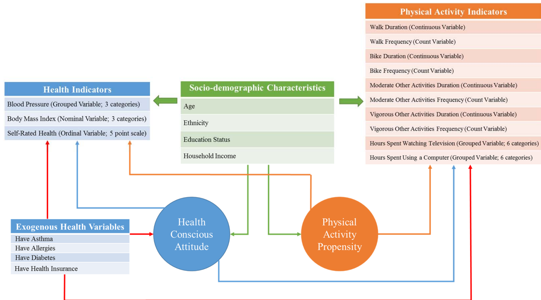
FIGURE 1. Model Framework
