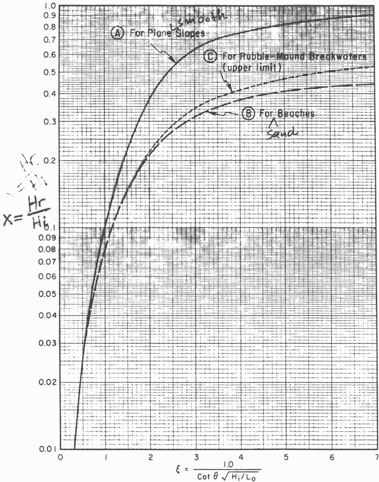
Figure 2-65. Wave reflection coefficients for slopes, beaches, and rubble-mound breakwaters as a function of the surf similarity parameter \xi .
