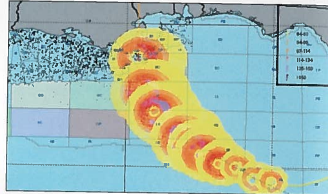
Figure 2: Hurricane wind fields of Katrina, 2005.
