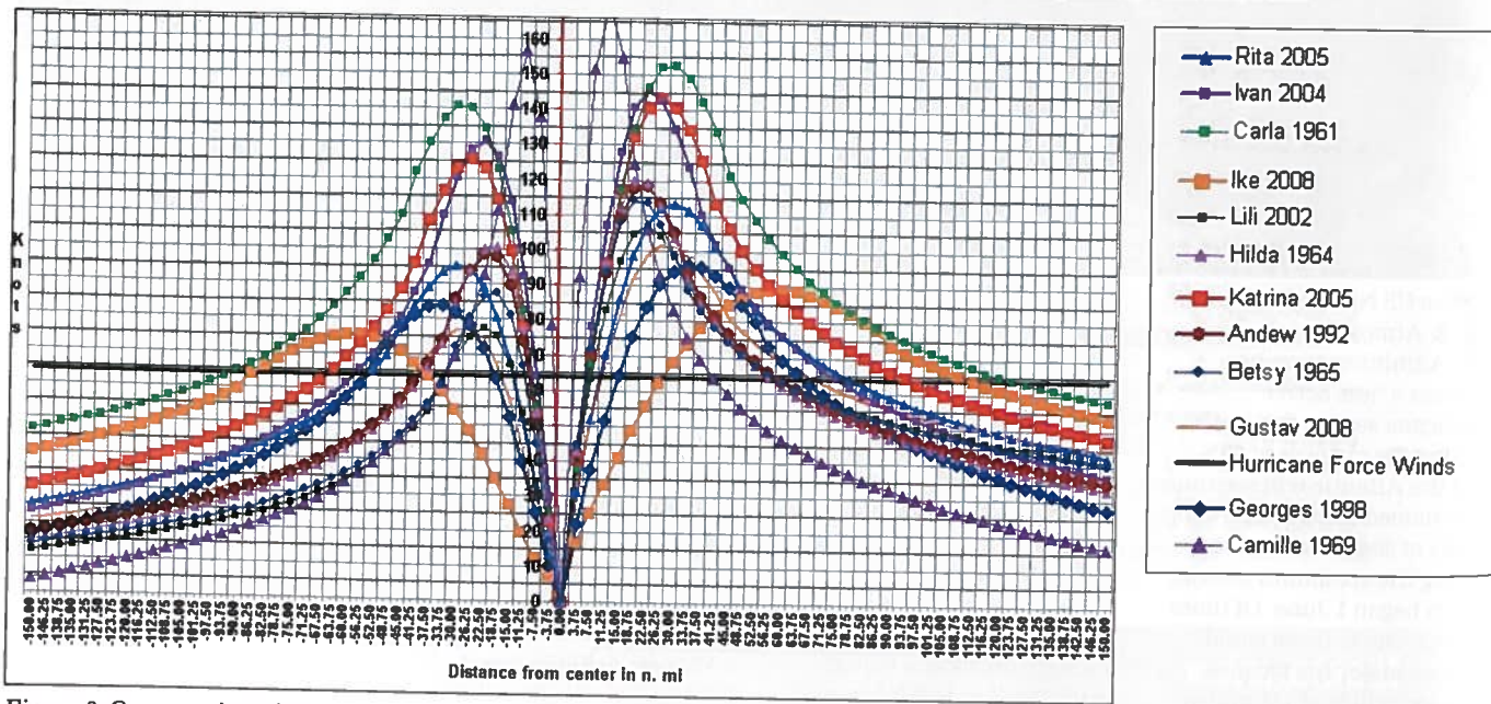
Figure 3: Cross-section of Gulf of Mexico hurricane wind fields.
