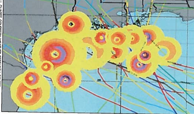
Figure 1: Wind fields of significant Gulf of Mexico hurricanes.
