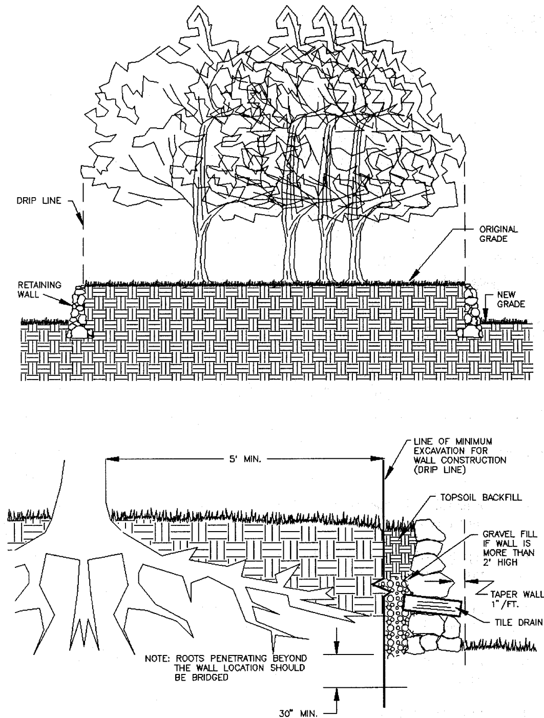
Figure 2-4 Example of a Tree Wall (VA Dept of Conservation, 1992)
