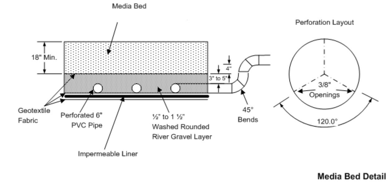
Figure 5-9: Illustration of optional outlet design
