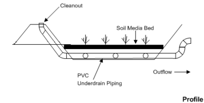
Figure 5-8: Detail of cleanout location
