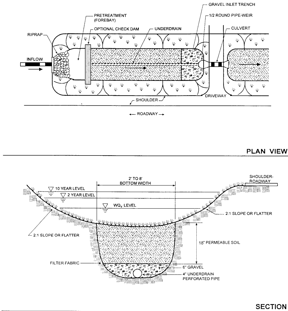
Figure 5-10: Diagram of Grassy Swale with Check Dam (MDE, 2000).
