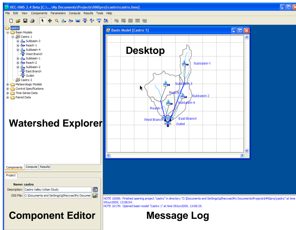
Figure 1. HEC-HMS user interface.
