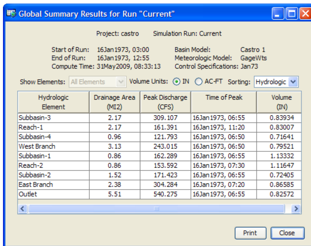
Figure 49. Viewing the global summary table.
