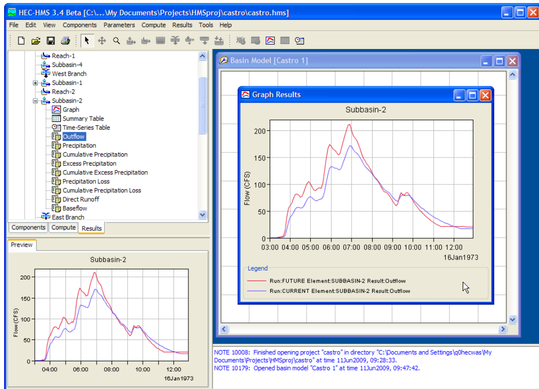
Figure 23. Comparing results from different simulation runs.
