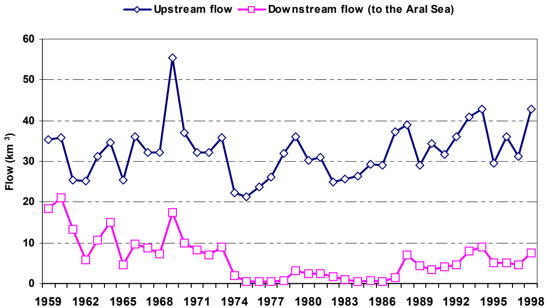
Figure 3—Upstream/downstream runoff of the Syr Darya River (Sources: Glantz (1999) for flows during 1959–88; Personal communication, V. Chub, Uzbekistan Main Hydromet, 2000, for flows during 1989–98.)
