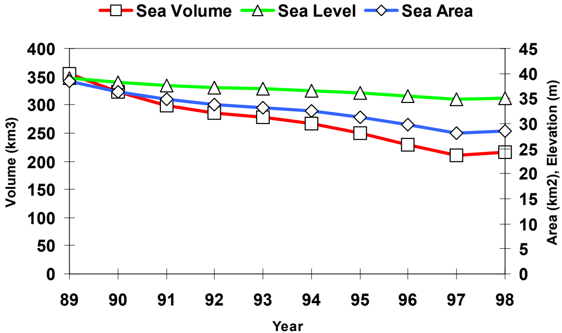
Figure 5—Change of level, area, and volume of the Aral Sea in recent years (Source: Personal communication, V. Chub, Uzbekistan Main Hydromet, 2000.)
